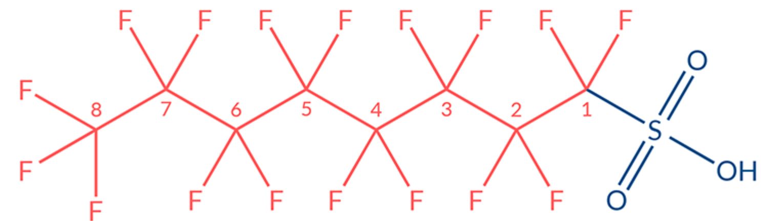
Perfluorooctanesulfonic Acid PFOS
