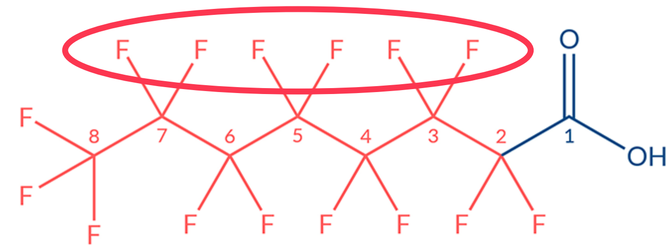
Pentadecafluorooctanoic Acid PFOA
